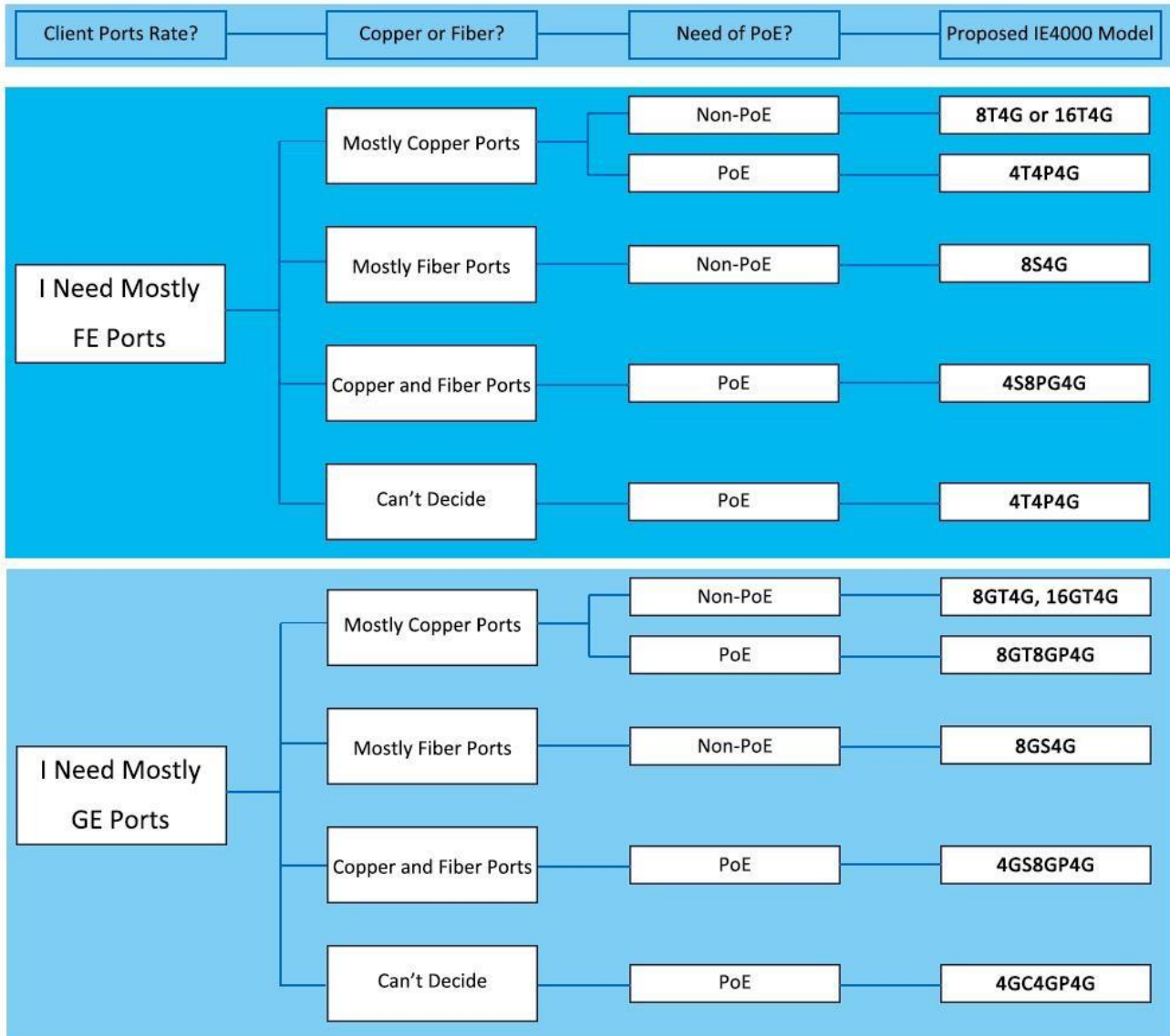
Figure 2. Cisco IE 4000 model selection guide
